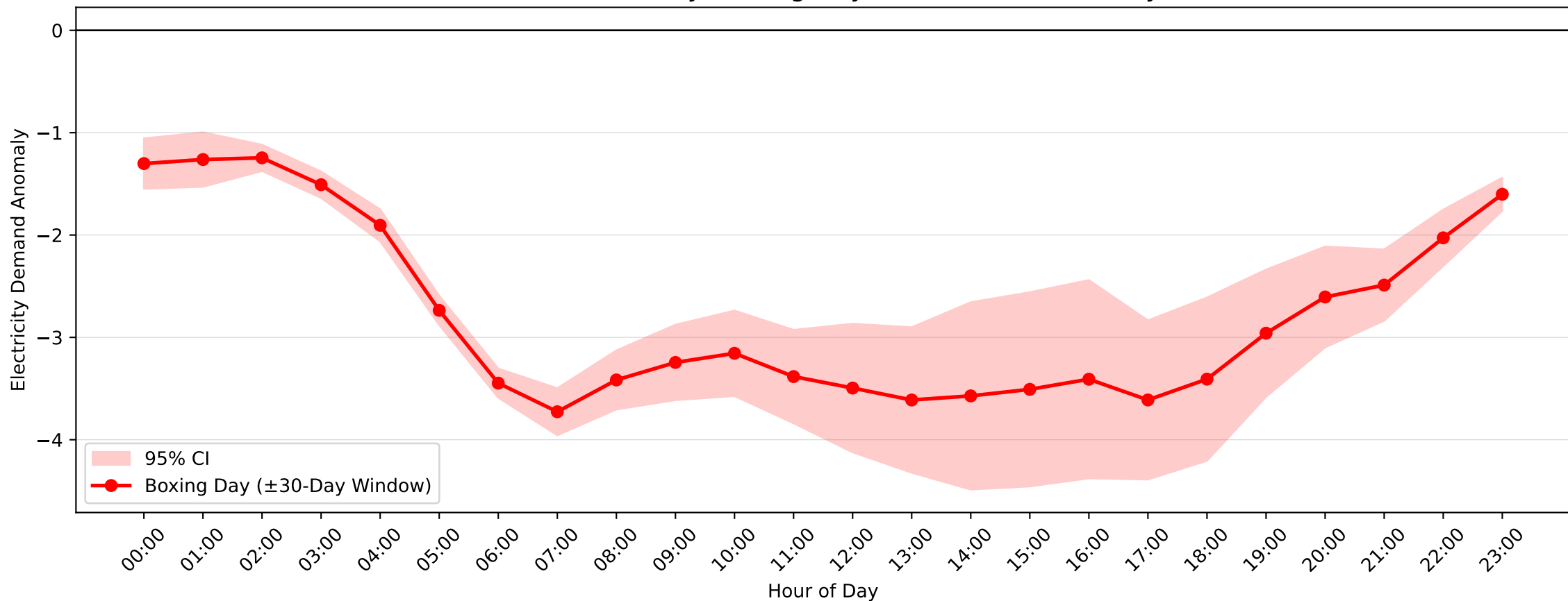
Lisarow Demand Anomaly: Boxing Day (2004–2017, \pm 30 -Day Window)
